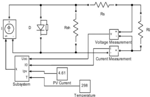
Fig.4. Solar PV module simulation model
