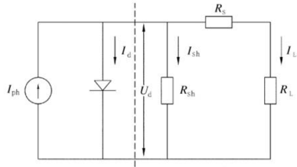
Fig.2. Photovoltaic cell equivalent circuit
