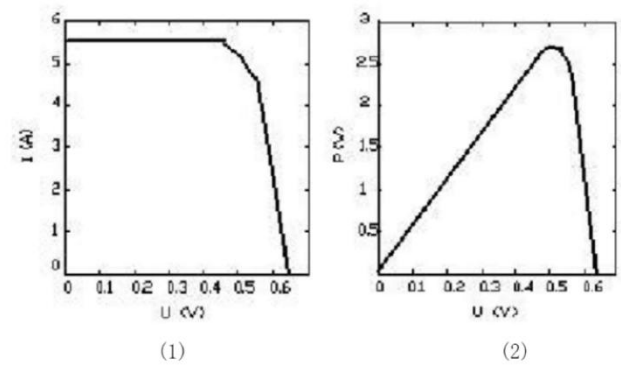
Fig.5. SOutput characteristic curve of a photovoltaic array
