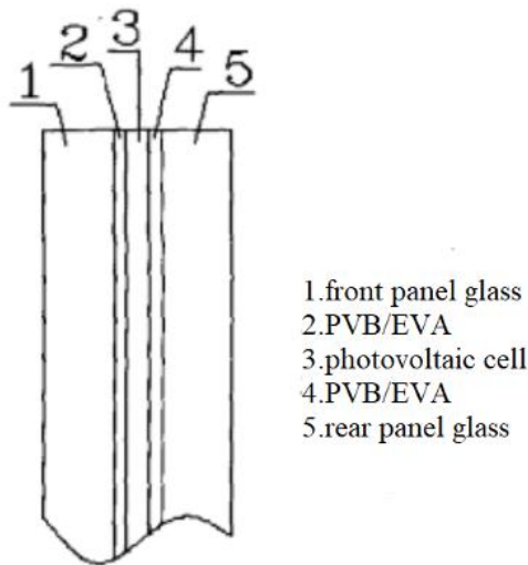
Fig.10. Double-layer clear glass photovoltaic module
