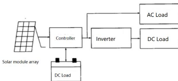
Figure.7. Schematic diagram of an independent photovoltaic greenhouse
