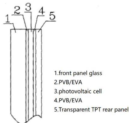
Fig.11 Single-layer transparent glass photovoltaic module.
