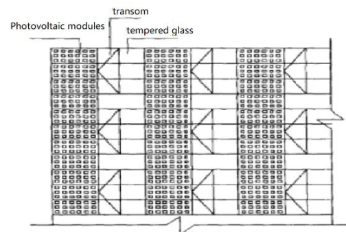
Fig.9. Floor plan of the photovoltaic greenhouse
